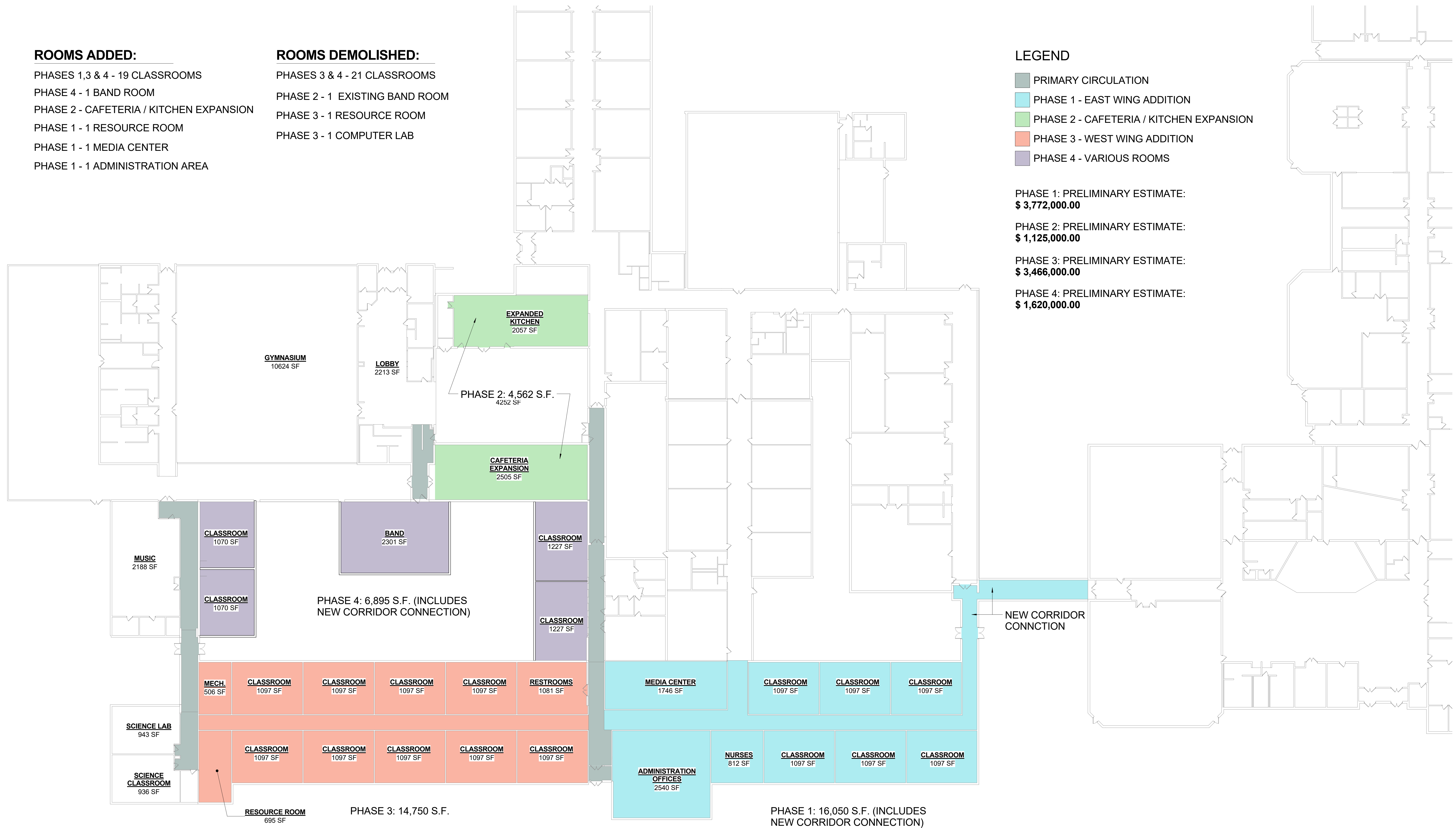
FLOOR PLAN - PHASE 4 3/64" = 1'-0"
