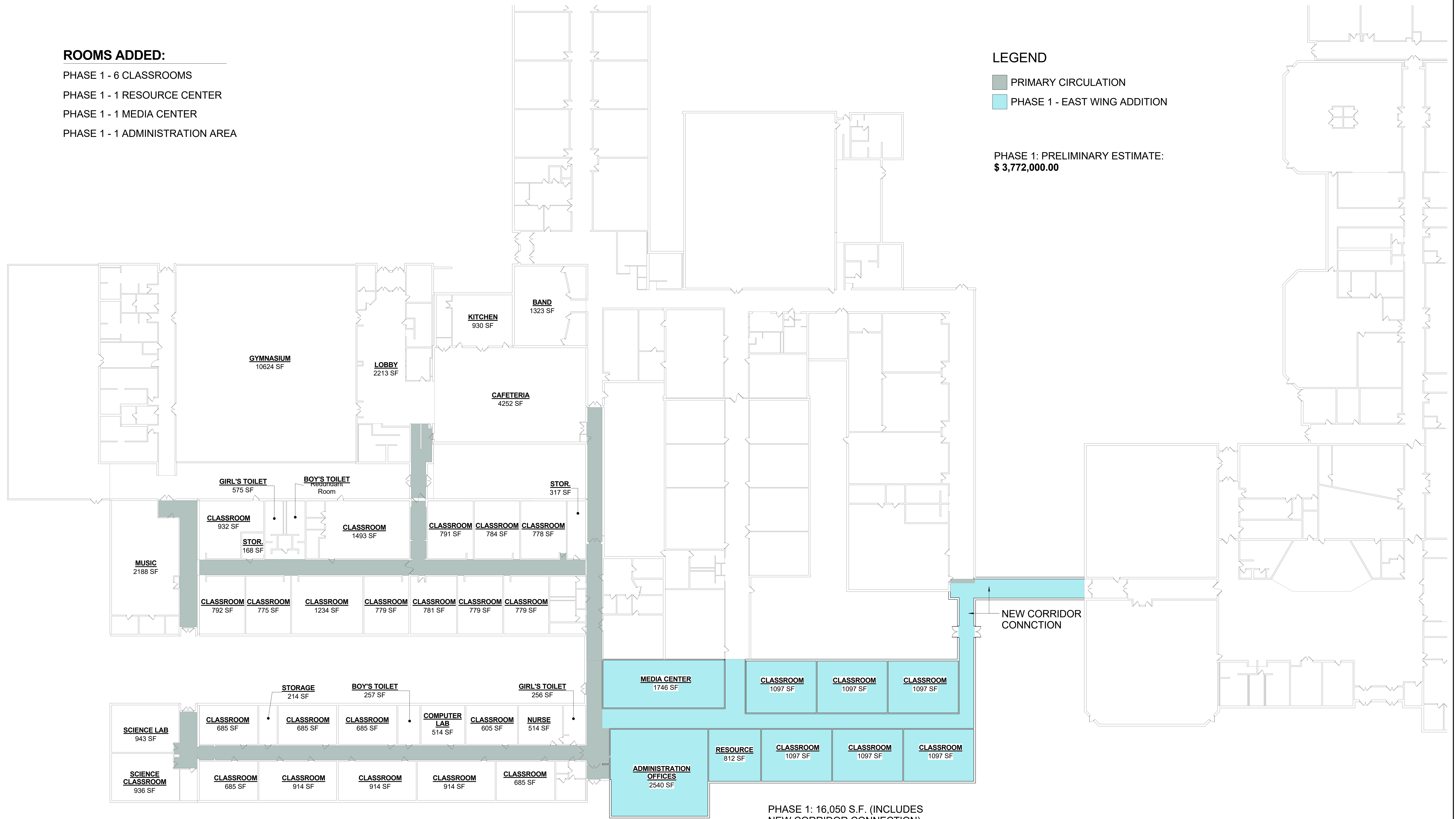
FLOOR PLAN - PHASE 1 3/64" = 1'-0"
