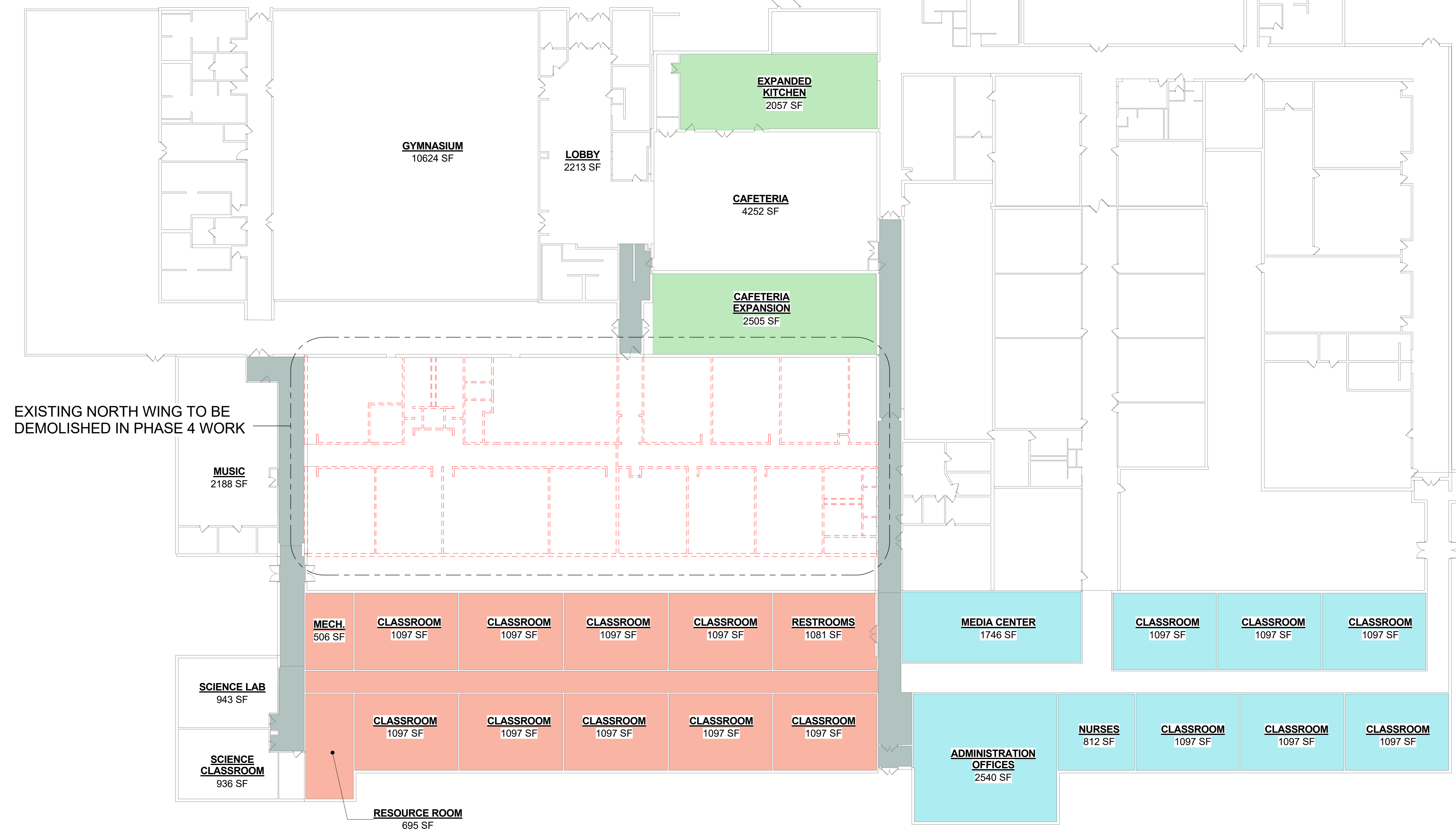
DEMOLITION FLOOR PLAN - PHASE 4 3/64" = 1'-0"
