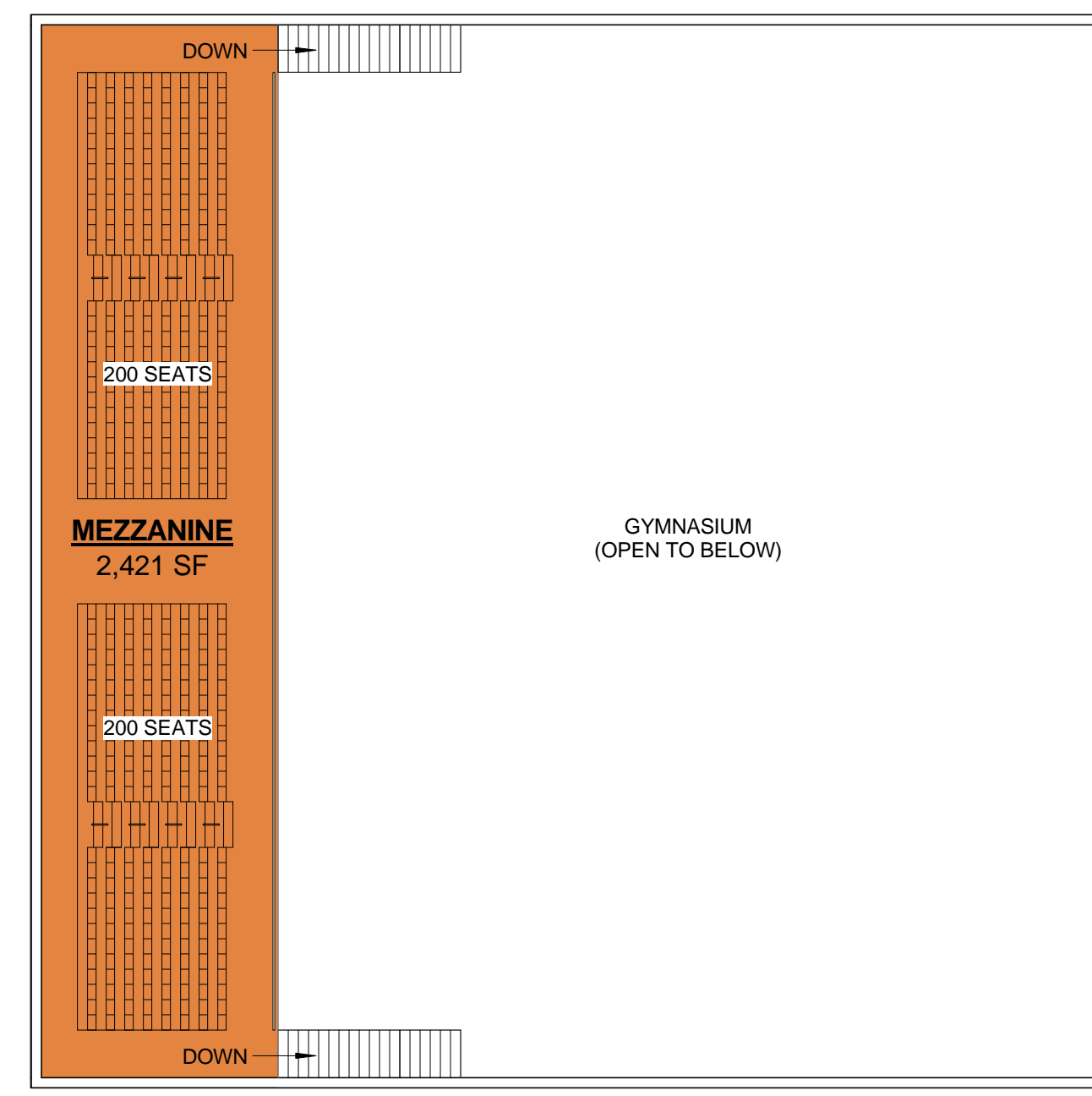
MEZZANINE PLAN
